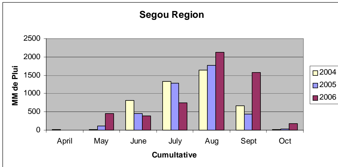
Figure 5 Rainfall in the region of Segou
